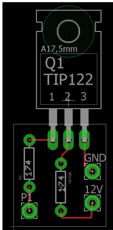
Figure 63 Power PCB Layout
