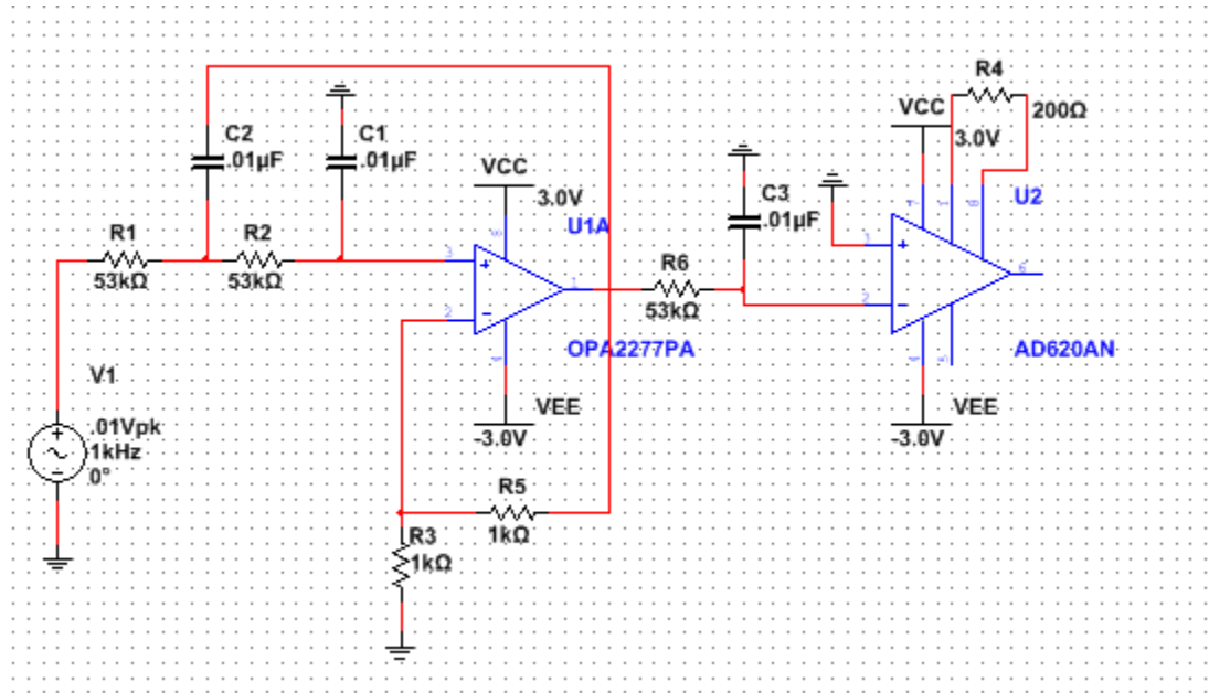
Figure 29 Microphone Schematic
