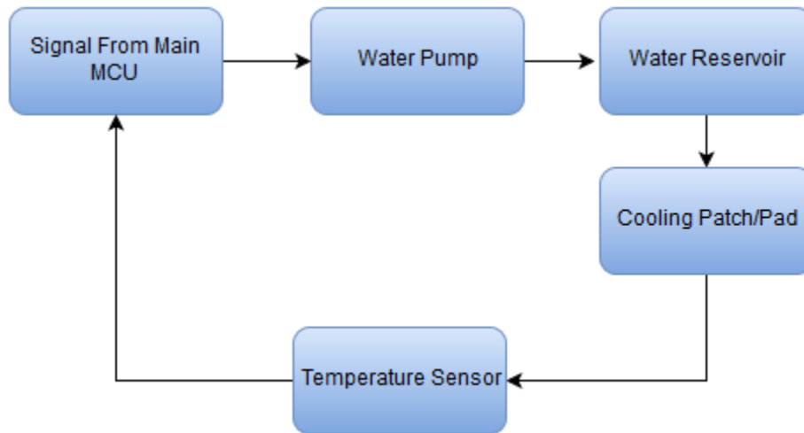
Figure 35 Cooling System Block Diagram
