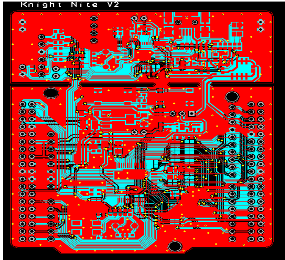
Figure 64 Final MCU PCB Layout
