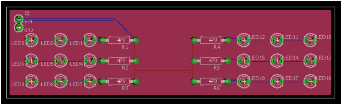
Figure 62 LED PCB Layout
