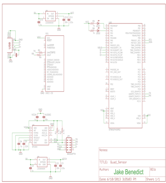
Figure 57 – MPU6050 implementation with STM32
