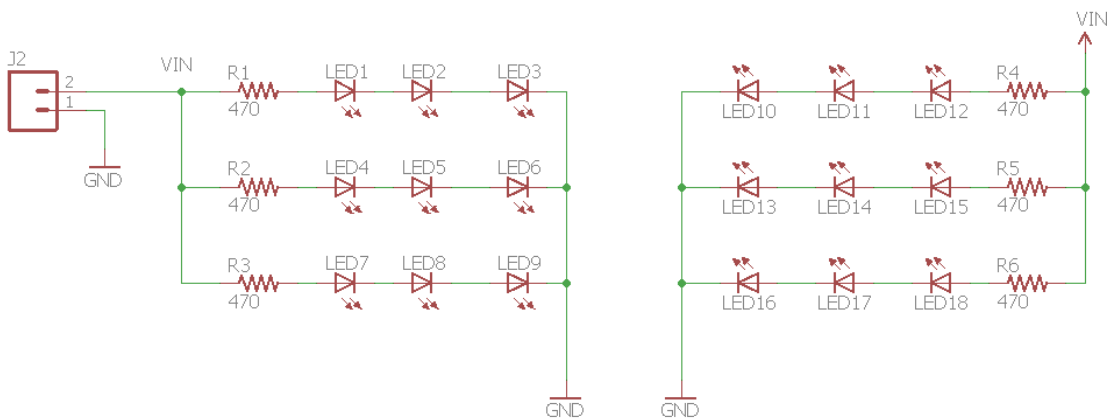
Figure 61 – LED Schematic
