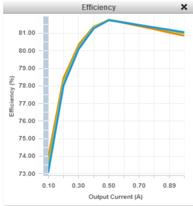
Figure 39 Efficiency
