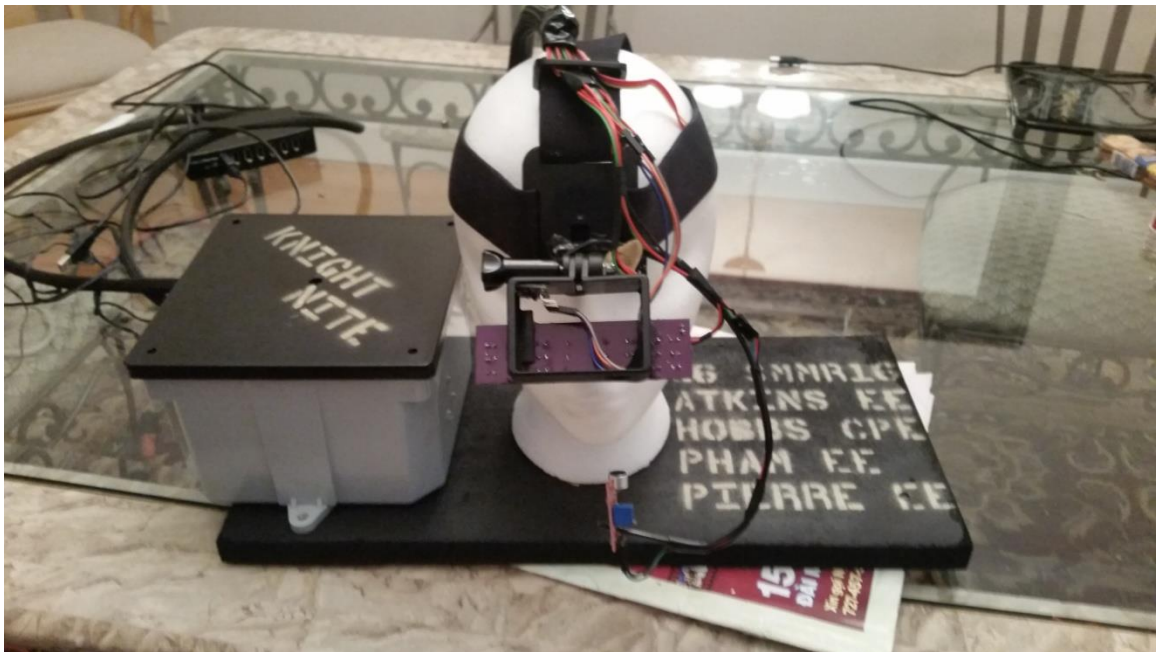
Figure 70 Final Knight Nite Prototype
