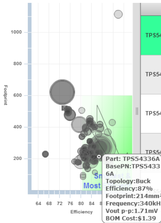
Figure 43 Topology Comparison
