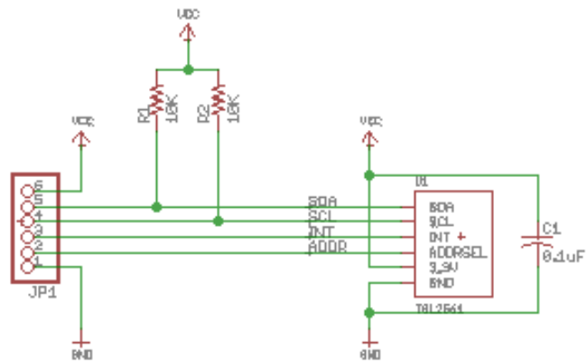
Figure 60 – Light Detection
