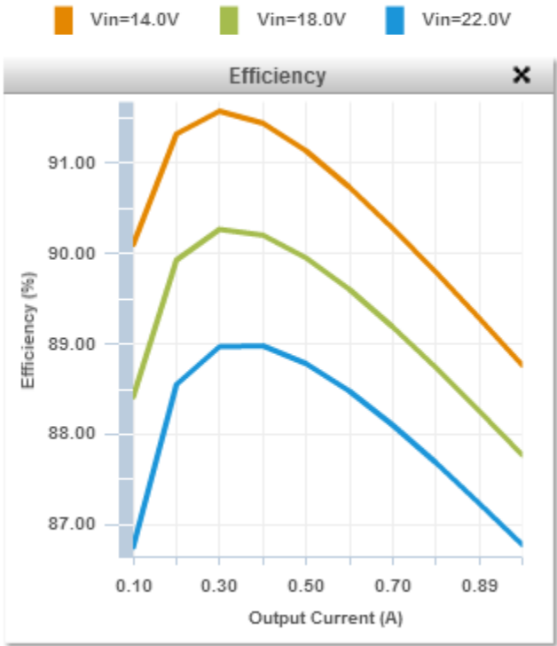
Figure 45 Efficiency
