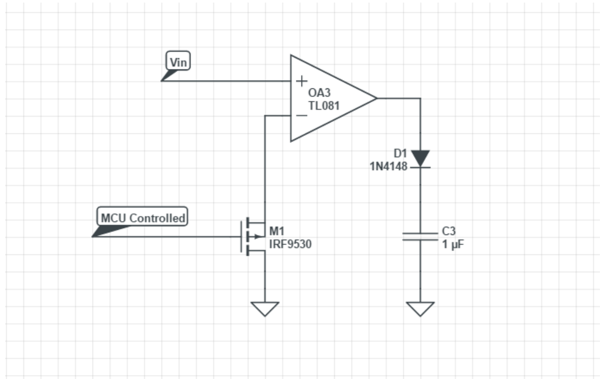
Figure 32 Peak detector circuit design
